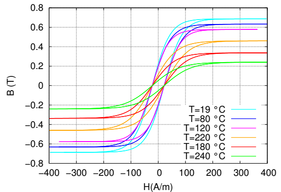
Fig. 2. Simulated hysteresis loops at different temperatures
