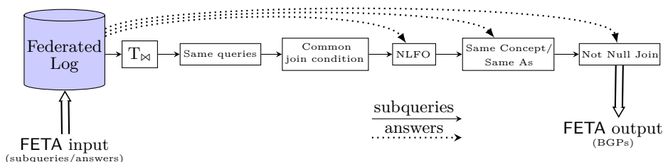
Fig. 3. Workflow processing of FETA's heuristics.
