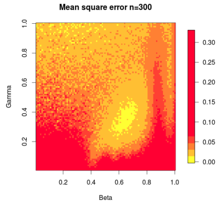
FIGURE 7. MSE in function of \beta and \gamma for absolut value function
