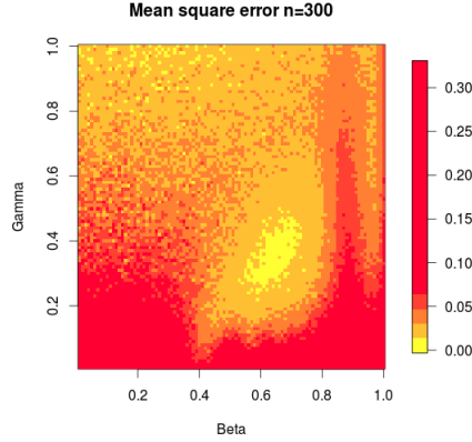
FIGURE 7. MSE for absolute value code
