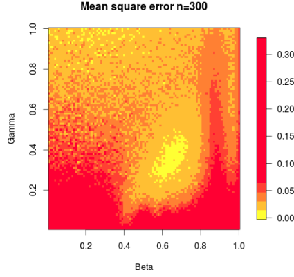
FIGURE 7. MSE for absolute value code
