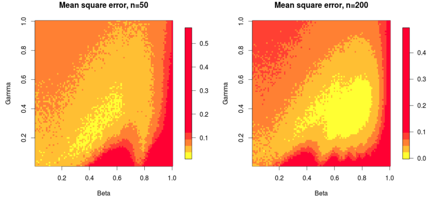
FIGURE 6. Mean square error in function of \beta and \gamma
