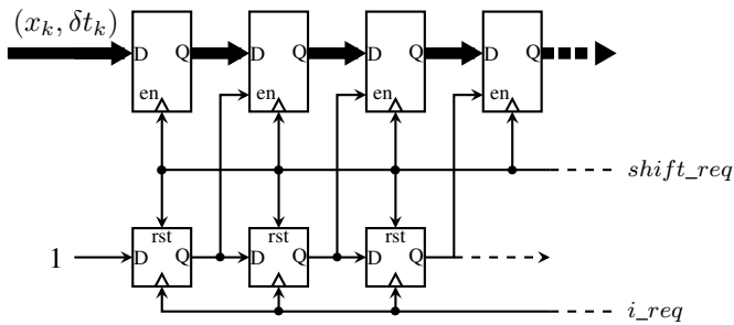
Fig. 11. Implementation details of the shift register.
