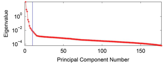
Fig. 3. Eigenvalues of \Upsilon for the HS image.
