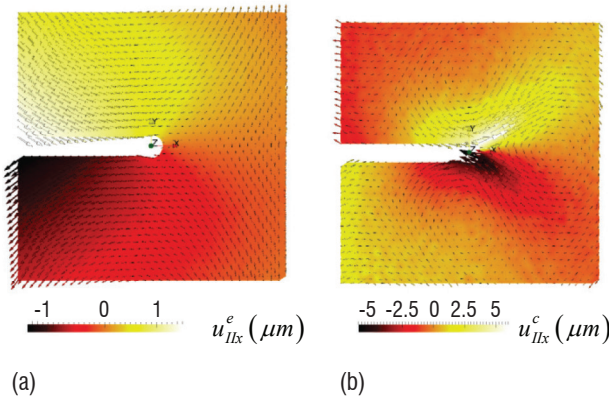
Figure 10 - Mode II reference fields constructed using DIC. Intensity of the component parallel to the crack plane. (a) Elastic reference field, (b) Non-elastic reference field.[10]
