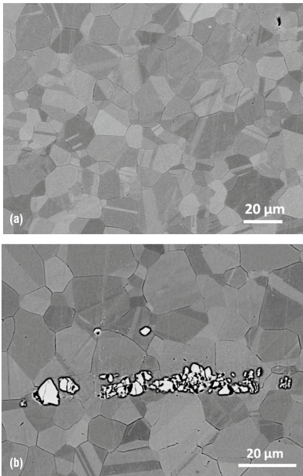
Figure 4 - Typical SEM micrographs of alloy 718 used in this study: (a) fully recrystallized equiaxed microstructure (b) typical carbide alignment in the rolling direction
