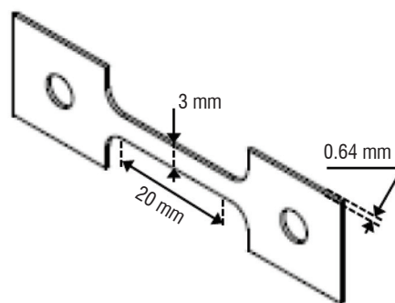
Figure 3 - Geometry of the tensile specimens used in this study
