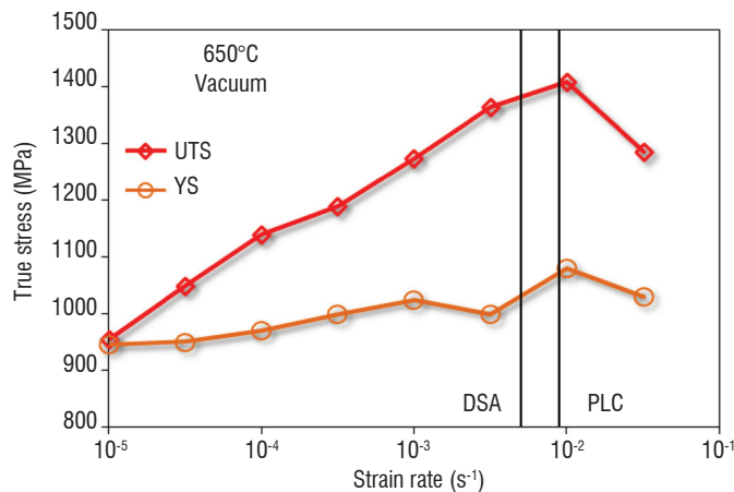
Figure 9 - Evolution of the yield stress and ultimate tensile stress for tensile tests at T=650^{\circ}\text{C} in a dynamic vacuum ( 10^{-5} mbar)
