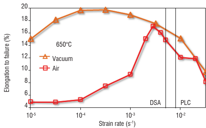
Figure 8 - Elongation to failure for tensile tests at T=650^{\circ}\text{C} for different types of atmosphere: dynamic vacuum ( 10^{-5} mbar), or air
