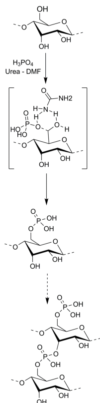
Scheme 6 Proposed mechanism by Nehls et al. 74 for the cellulose phosphorylation with H_3PO_4 in presence of urea. The substitution preferentially occurs in the C-6-position and is potentially followed by cross-linking.
