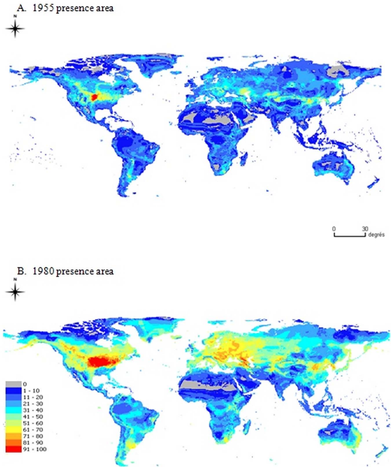
Figure 5. Outputs of model ES obtained with 20 presence data located within the 1955 presence area (A) and with 50 presence data located within the 1980 presence area (B). The model was fitted using 19 input variables in both cases. doi:10.1371/journal.pone.0020957.g005
