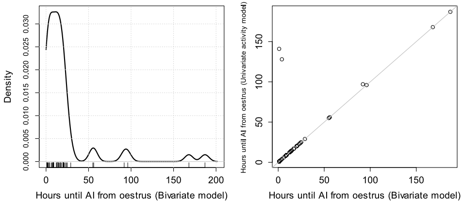
Figure 7. Left: Kernel density estimate of the time difference between successful AI and the most recently detected oestrus state by the bivariate model. Right: The univariate model against the bivariate model for time to successful AI from detected oestrus. Note the two large values from the univariate model, certainly false negatives.
