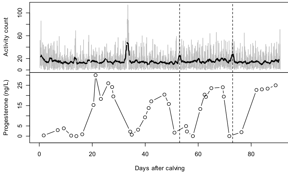
Figure 1. Top: The raw hourly activity counts from a pedometer against time since calving (grey), the black line is as 24-hour centred moving average. Bottom: The progesterone concentration over the same time and cow. The dashed vertical lines are times when an artificial insemination occurred (an indicator of oestrus). Note that these occur after a drop in progesterone and during a brief spike in activity levels.
