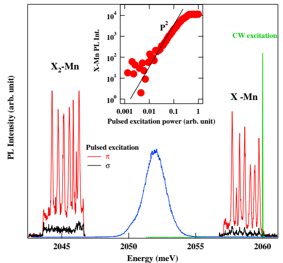
FIG. 8: PL spectra of a Mn-doped QD obtained under a two-photon resonant absorption of a picosecond laser pulse (spectra of the pulsed laser in blue). The resonant creation of the biexciton (X 2 -Mn) is only possible for a linearly polarized excitation (red) whereas almost no PL is observed for circularly polarized pulses (black). The influence on the Mn spin population of a CW control laser (spectra of the CW laser in green) in resonance with the exciton (X-Mn) levels can be detected in the intensity distribution of X 2 -Mn. Inset: PL intensity of X-Mn versus the intensity of the pulsed linearly polarized excitation. The P^2 dependence is characteristic of a two-photon absorption.
