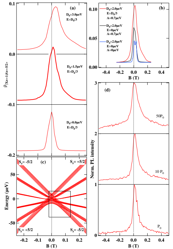
FIG. 13: (a) Modelling of the longitudinal magnetic field dependence of the population of the exciton state |X_z = -1, S_z = -5/2\rangle under resonant excitation for different values of the crystal field terms D_0 and E=D_0/3 (the curves are vertically shifted for clarity). The population of this level is proportional to the resonant PL signal. The parameters used in the calculation (see text for details) are \hbar\Omega_R = 15\mu\text{eV} , \tau_{Mn} = 100\text{ns} , \tau_r = 0.3\text{ns} , \tau_{relax} = 50\text{ns} , \tau_d = 100\text{ps} , A = 0.7\mu\text{eV} , a = 0.32\mu\text{eV} and g_{Mn} = 2 . (b) Calculated population of the exciton state |X_z = -1, S_z = -5/2\rangle for D_0=2\mu\text{eV} and E=D_0/3 (red), E=0 (black), E=0 and A=0 (blue). (c) Calculated fine and hyperfine structure of a Mn spin with A = 0.7\mu\text{eV} , a = 0.32\mu\text{eV} , g_{Mn} = 2 , D_0=1.5\mu\text{eV} and E=D_0/3 . The black rectangle highlights the magnetic field range where the state S_z=-5/2 significantly interacts with the other Mn spin states. (d) Experimental magnetic field dependence of the resonant PL signal for different excitation intensities and \sigma- excitation / \sigma+ detection on the high and low energy lines respectively. The curves are normalized and vertically shifted for clarity.
