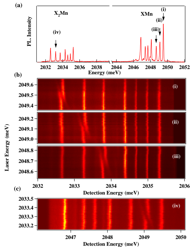
FIG. 6: (a) PL of the exciton and biexciton in a Mn-doped QD. (b) Autler-Townes splitting of the exciton detected on the biexciton PL under resonant excitation of the ground-to-exciton transition for the spin state of the Mn S_z = +5/2 (i), S_z = +3/2 (ii) and S_z = +1/2 (iii) (arrows in the PL spectra). (c) Emission of the exciton for a dressed exciton-to-biexciton transition. The excitation is tuned around the state S_z = +3/2 of the biexciton (iv).
