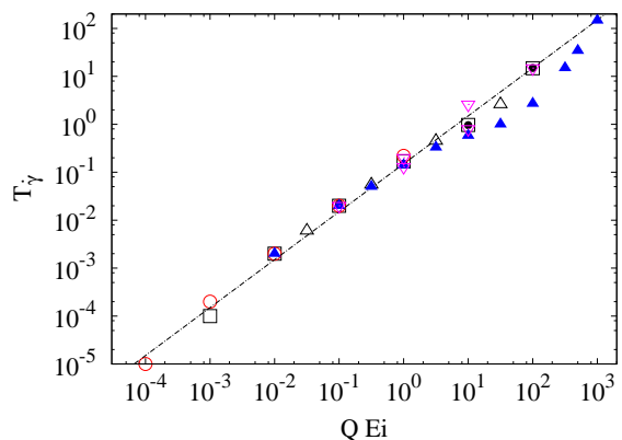
FIG. 3. Shear contribution T_\gamma = T_K - T_0 to the kinetic temperature measured in underdamped samples vs. Q Ei . (▽) Data at T_0 = 0.2 . The line represents T_\gamma = 0.15 \cdot Q \cdot Ei .
