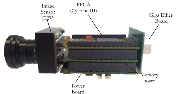
Fig. 1: DreamCam system
