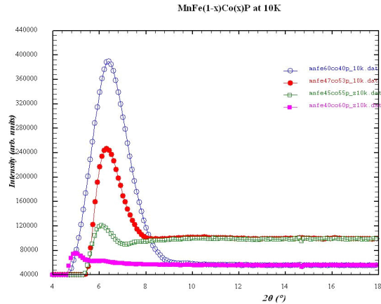
Figure 4. Variation of the small angle maxima (0,0,q(x)) recorded at 10 K for selected x cobalt contents.
