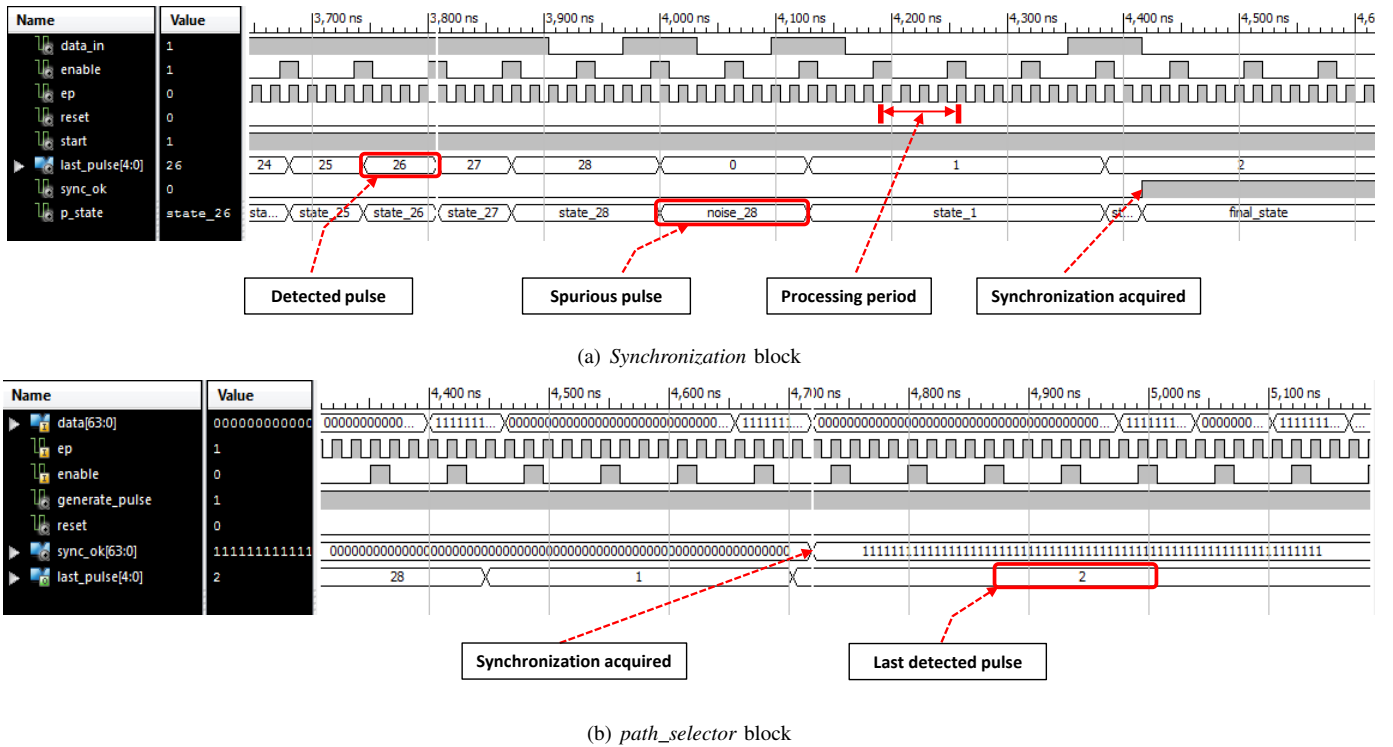
Fig. 8. Example of signal waveform results of the implemented hardware synchronization architecture
