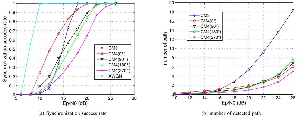
Fig. 7. Simulation results of the proposed algorithm for various channel models
