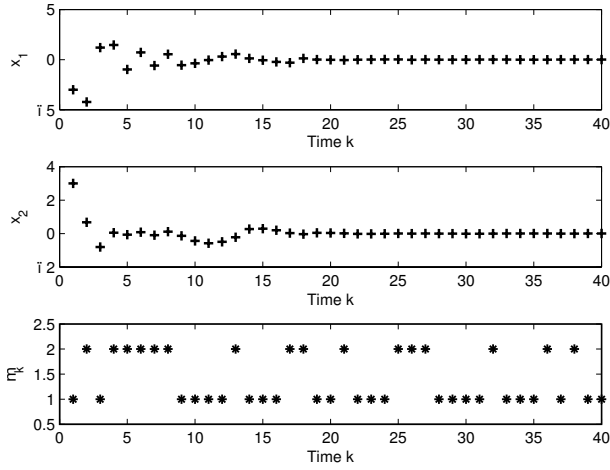
Fig. 6. State evolution and min-switching control (24)-(26).
