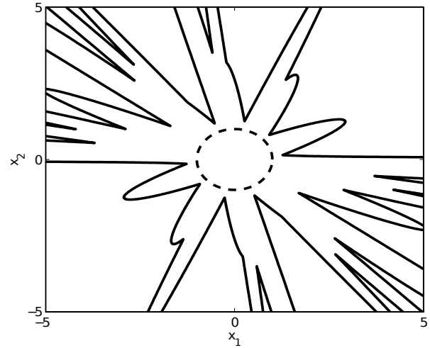
Fig. 4. Sets \mathcal{B} (dashed) and \bigcup_{i \in \mathcal{S}[1:7]} \mathcal{B}_i (solid).
