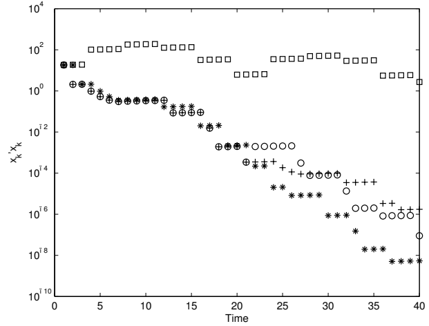
Fig. 9. Comparison between the evolution of the Euclidean norm of the state for the different switching laws: induced by geometric condition (4) (star); min-switching law (24)-(26) (cross); min-switching control (30) (circle) and periodic rule (square).
