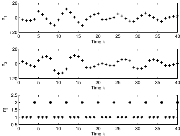
Fig. 8. State evolution and periodic switching control with M = 4 .
