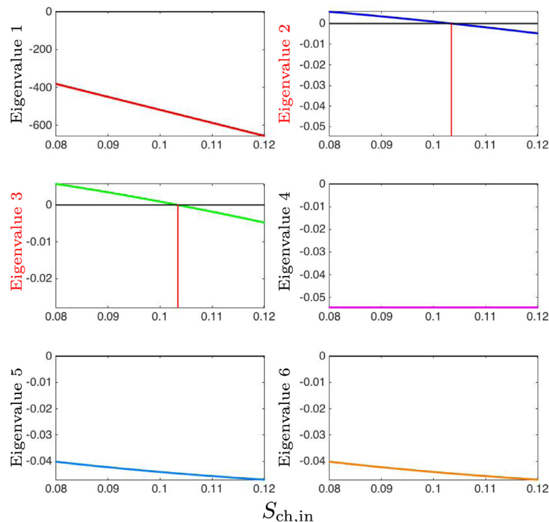
Fig. B.14. Real parts of the eigenvalues determined at D = 0.01 and S_{ch, in} = [0.08, 0.12] , in the case with maintenance. The red vertical lines indicate the location where the eigenvalue crosses zero. (For interpretation of the references to colour in this figure legend, the reader is referred to the web version of this article.)
