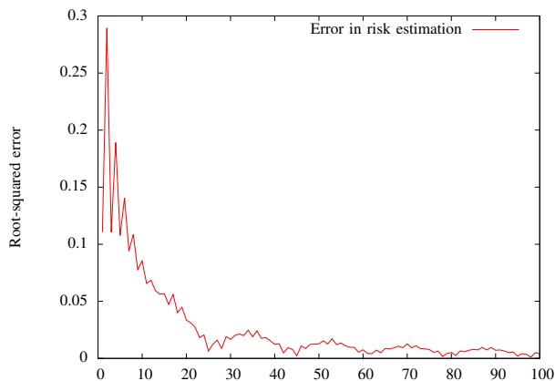
Fig. 4. Approximation error of the trapezoidal rule with regard to the number of trapezoids (i.e., segments) used for numerical integration when computing the unsupervised risk.
