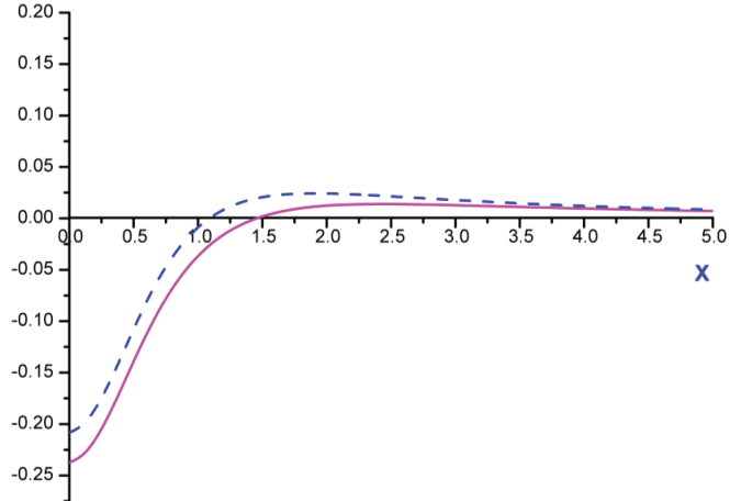
Figure 3. Function f_{2-\alpha}(x) —dashed line. The solid line is the behavior of f_{2-\alpha}(x; \varepsilon = 1) , obtained in numerical calculations accounting for the collapse effect [24].
