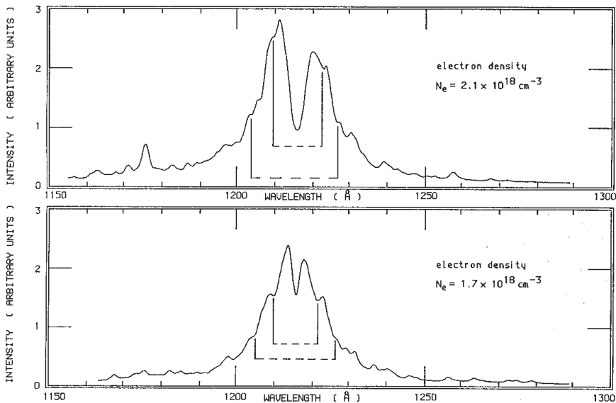
Figure 2. Comparison of the experimental and theoretical positions of the dips in the profiles of the hydrogen Ly \alpha line in the gas-liner pinch. The theoretical positions are shown by vertical solid lines connected by dashed lines.
