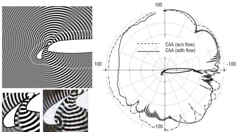
Figure 13 - Noise radiation by the slat cove trailing edge of a high lift wing at approach, as predicted by a CAA calculation based on an equivalent (analytical) source. Left side; instantaneous perturbed pressure field obtained over the domain (top) or within the slat cove (bottom left), to be compared with near-field CFD results obtained for an alternative configuration (bottom right, calculation by NASA). Right side; mid-field directivity diagram (in lines, to be compared with its quiescent medium radiation counterpart, in dashes). Reproduced from [20] with permission
