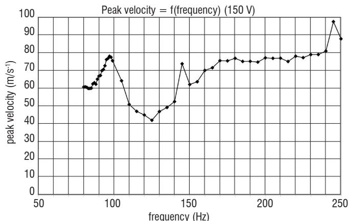
Figure 24 - Peak velocity as function of forcing frequency for 150 V
