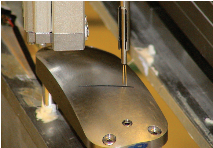
Figure 27 - Hot-wire qualification of an actuator as a wind tunnel model component
