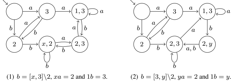
Fig. 39: 3MSA for the case in which condition 3. of Proposition 25 is false.
