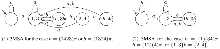
Fig. 2: 3MSA for automata that do not satisfy conditions 1. and 2. of Proposition 9.
