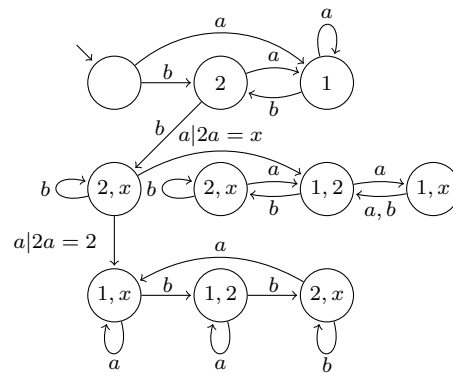
(2) 3MSA for the case b = [x, 1] \setminus 2 , 2b = x \{2a, xa\} = \{2, x\} and \{2ab, xab\} = \{1, x\} .
