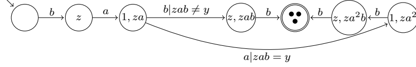
Fig. 37: P3MSA for the case b = [x, y] \setminus z , \{x, y\} = \{1, 2\} and |Orb_a(z)| > 2 .
