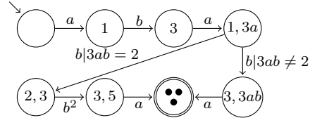
(2) P3MSA for the case b = (13)(245\dots)\pi .
