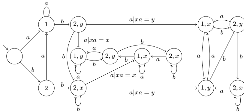
(3) 3MSA for the case b = [x, y] \setminus 2 , 2b = x , 1b = y , 1 \notin \{x, y\} and \{xa, ya\} = \{x, y\} .
