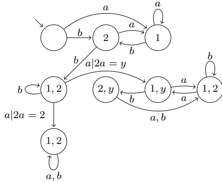
(1) 3MSA for the case b = [1, y] \setminus 2 , 2b = 1 , Orb_a(2) \subseteq \{2, y\} and 2ab \in \{1, y\} .
