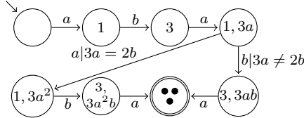
(1) P3MSA for the case b = (13)(2)\pi or b = (13)(24)\pi , and \{2b, 3\}a \neq \{2b, 3\} .
