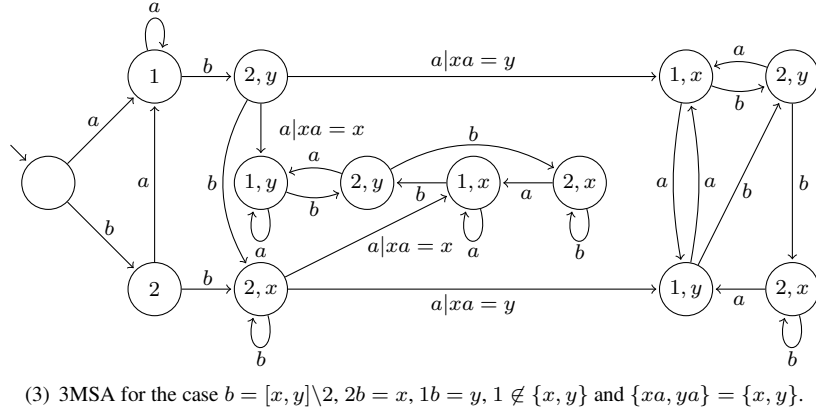
Fig. 31: 3MSA for the case in which condition 2. of Proposition 22 is false.
