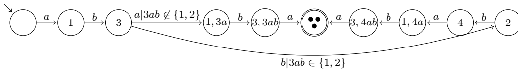
Fig. 11: P3MSA for the case b = (1324)\pi and \{3, 4\}a \neq \{3, 4\} .
