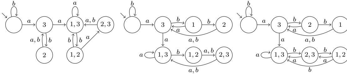
(1) 3MSA for the case b = (1)(23)\pi and 2a = 2 . (2) 3MSA for the case b = (123)\pi and 2a = 2 . (3) 3MSA for the case b = (132)\pi and 2a = 2 .
