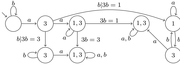
(1) 3MSA for the case \{1, 3\}b = \{1, 3\} .
