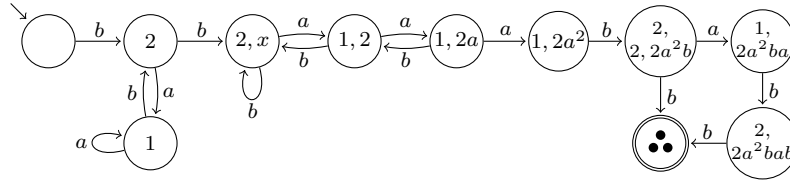
Fig. 34: P3MSA for the case b = [x, 1] \setminus 2 , 2ab = 1 , xab = x and \{2a, xa\} \neq \{2, x\} .
