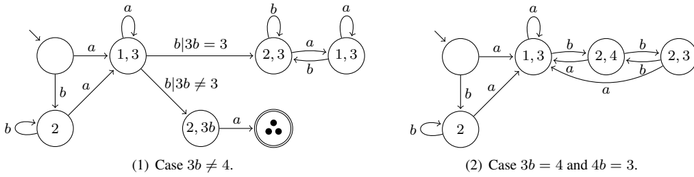
Fig. 24: 3MSA for automata that do not satisfy condition 3. of Proposition 14 with y = 1 .
