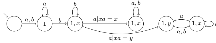
Fig. 29: 3MSA for the case in which condition 1. of Proposition 22 is false.
