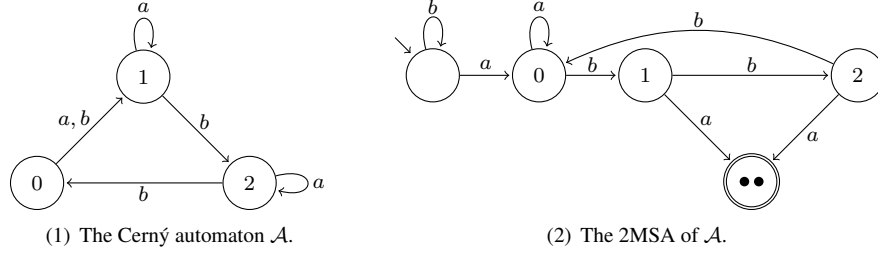
Fig. 1: The Cerný semiautomaton with 3 states and its 2MSA: the set of synchronizing words for \mathcal{A} is the regular language b^*a^+(b^3)^*(b+b^2)a(a+b)^* .
