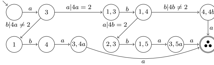
Fig. 18: P3MSA for the case b = (314\dots)\pi .
