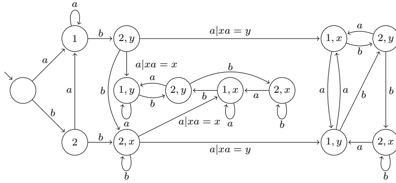
(3) 3MSA for the case b = [x, y] \setminus 2 , 2y = x , 1b = y , 1 \notin \{x, y\} and \{xa, ya\} = \{x, y\} .
