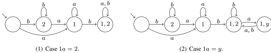
Fig. 26: 3MSA for automata that do not satisfy conditions 1. and 2. of Lemma 16 with 1b = 1 .
