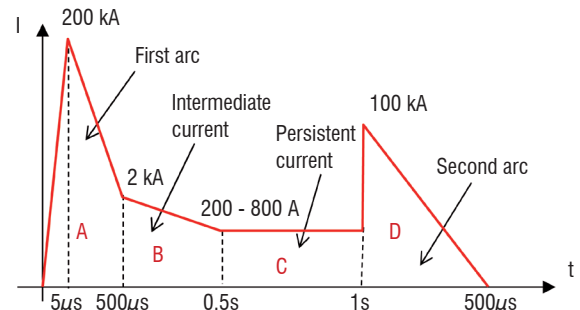
Figure 1 - Typical arc lightning waveform, as defined in the RTCA [4] and EUROCAE [15]
