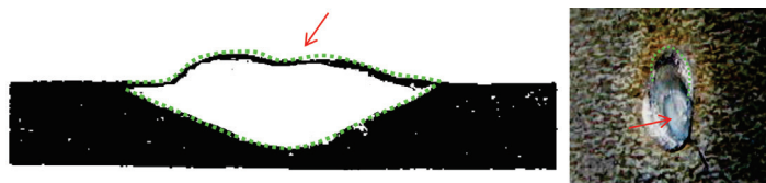
Figure 18 - Picture on the left, section through the center of the cathode spot (Dobbing & Hanson, 1978). Picture on the right, view of a cathode spot for an 800A, 200C arc on an aluminum panel (DGA-TA). The drop of metal is deformed by gravity.
