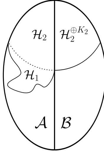
FIGURE 2. The structure of a \emptyset -closed subset of \mathcal{G}_1
