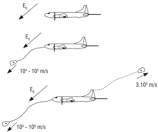
Figure 10 – Lightning triggering scenario. E_0 is the ambient atmospheric electric field. A positive leader merges from the front part of the aircraft and propagates in the direction of the atmospheric field. It induces a negative charge on the aircraft, increasing the local field on the rear part of the aircraft, from which a negative leader starts its propagation. The total charge of the positive leader, the negative leader and the aircraft is neutral.
