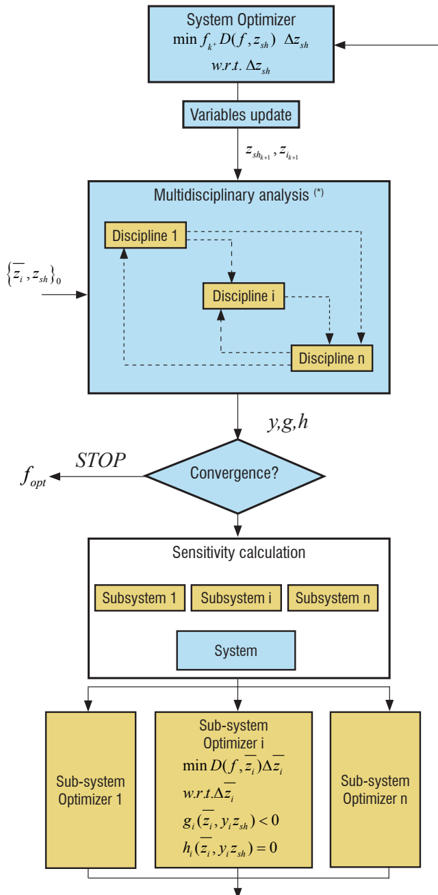
Figure 6 – BLISS (*)MDA is optional and allows to have a consistent starting point
