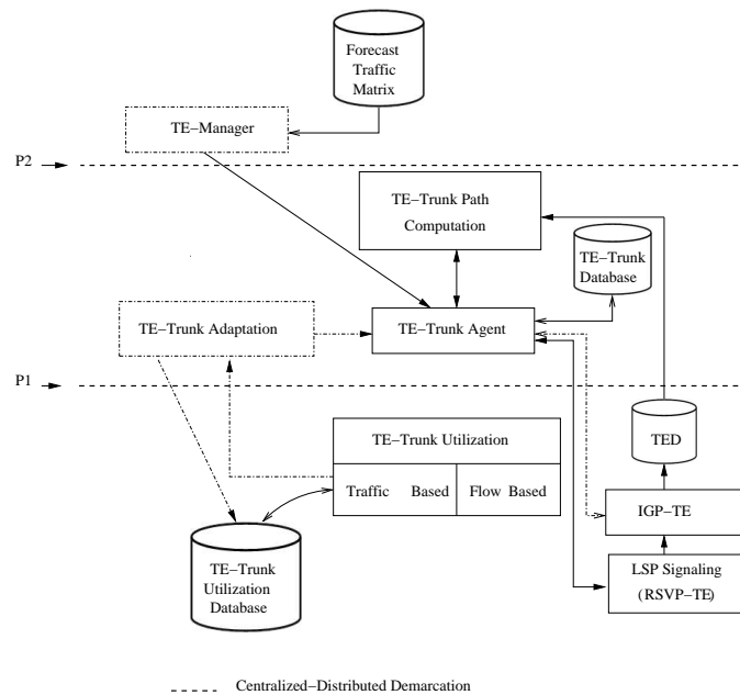
Figure 2. The Off/Cen/Coo and On/Dis/Unc MPLS-TE mechanisms
