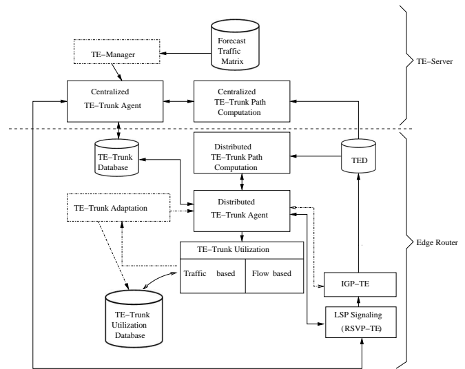
Figure 3. Hybrid MPLS-TE Approach
