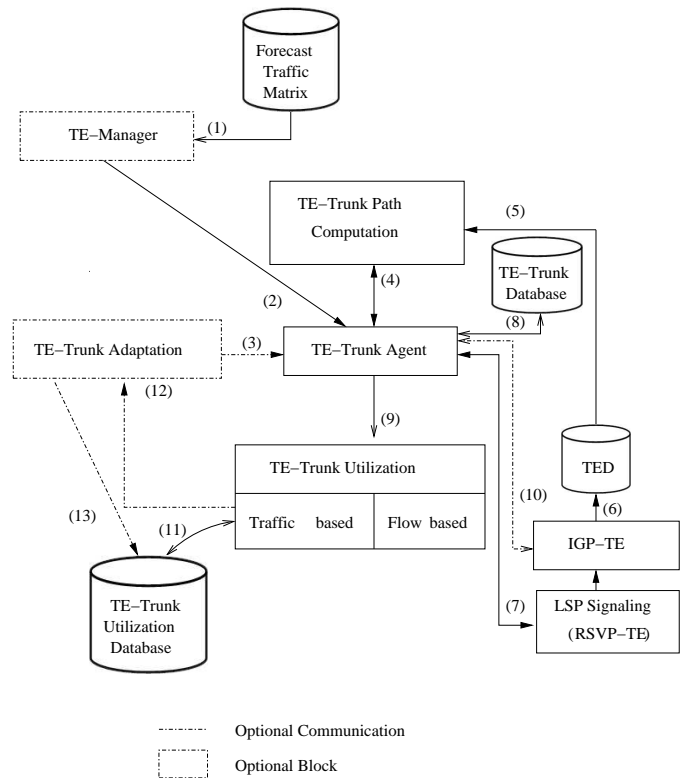
Figure 1. Generic architecture for MPLS-TE Routing Systems
