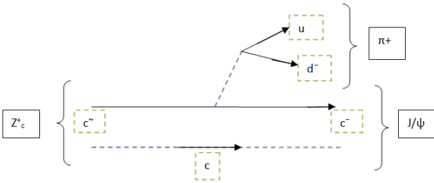
Fig. 2. An ECS-quark description of Z_c decay. The ECS-favored process is \tilde{c} \rightarrow \bar{c}ud with a spectator c quark.
