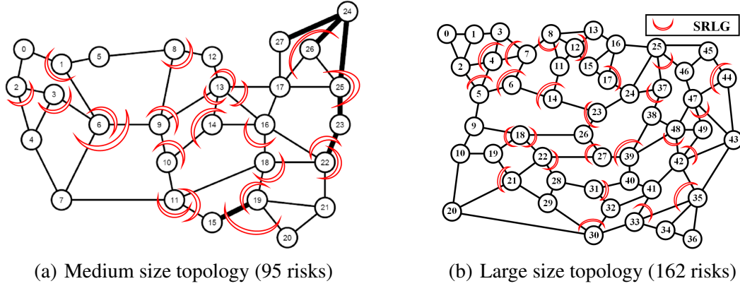
Fig. 5. Test topologies
