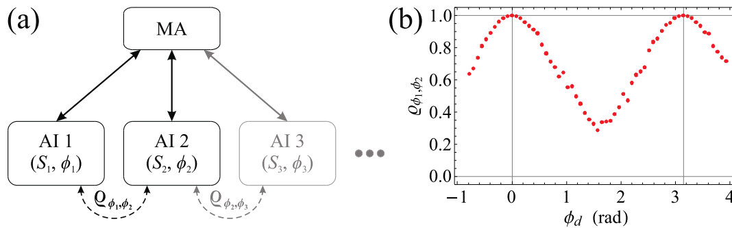
Figure 3. (a) Schematic illustrating the source of correlation in the differential FRAC method. The signal from each atom interferometer (AI), exhibiting a known scale factor S_j and unknown phase shift \phi_j , is directly correlated (indicated by the solid lines) with a common vibration phase measured by a mechanical accelerometer (MA). Since the resulting fringes are derived from a common source, measurements of each \phi_j are highly correlated, as indicated by the dotted lines and characterized by the positive coefficient \rho_{\phi_i, \phi_j} . This technique can be extended for multiple coupled interferometers (shown in gray), although we focus on the case of only two. (b) Correlation coefficient \rho_{\phi_1, \phi_2} as a function of \phi_d estimated from a large sample of simulated fringes. Here, we assumed \kappa = 1 and we added non-common Gaussian noise to the phase of the reconstructed fringes with a standard deviation of \sigma_{\phi_d} = 0.1 rad.
