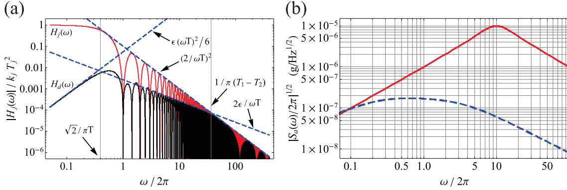
Figure C2. (a) Normalized transfer functions, |H_j(\omega)|/k_j^{\text{eff}} T_j^2 , described by eq. (C.10) for coupled K-Rb interferometers. These functions determine the response of the single-species (red curve) and dual-species (black curve) interferometers to acceleration noise at different frequencies, \omega . Here, T_1 = 1 s and T_2 = (1 - \epsilon)T_1 , with \epsilon = 1 - \sqrt{k_1^{\text{eff}}/k_2^{\text{eff}}} \simeq 0.0087 , and \tau_1 = \tau_2 = 10 \mu\text{s} . (b) Model curves for the power spectral density of ground vibrations described by eq. (C.13). The solid red curve corresponds to the power spectral density of a “quiet” location [66, 67] that we simulated with the parameters \xi = 0.5 , \chi = 1 , \omega_0/2\pi = 10 Hz, a_{\text{rms}} = 1.4 \times 10^{-4} g. The dashed blue curve corresponds to “low-noise” conditions achievable with passive vibration isolation ( \xi = 2 , \chi = 0.8 , \omega_0/2\pi = 1 Hz, a_{\text{rms}} = 1.4 \times 10^{-6} g). These two curves were used to compute the rms phase noise in table 1.
