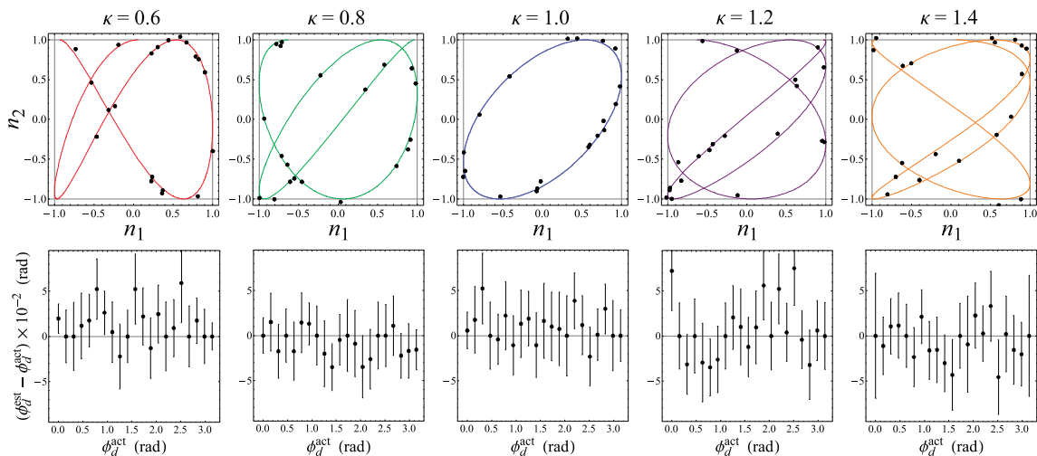
Figure B2. Simulated Bayesian phase estimates in the presence of offset noise. Top row: simulated data for \kappa = \{0.6, 0.8, 1.0, 1.2, 1.4\} . Here, points based on eq. (B.3) were generated from common phases chosen randomly over the range \phi_c \in [-2\pi, 2\pi] . The differential phase was set to \phi_d^{\text{act}} = 1 rad, and offset noise was applied to the points via Gaussian distributions with standard deviations \{\sigma_{B_1}, \sigma_{B_2}\} = \{0.02, 0.04\} —corresponding to \text{SNR} \sim 50 and 25 , respectively. Bottom row: the systematic error in the Bayesian phase estimate, \phi_d^{\text{est}} - \phi_d^{\text{act}} , as a function of \phi_d^{\text{act}} for each value of \kappa . Only 10 points were required to bring the statistical uncertainty indicated by the error bars to \lesssim 50 mrad.
