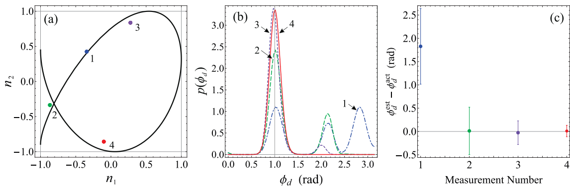
Figure 1. The process of Bayesian estimation of the differential phase \phi_d from synthetic data following a Lissajous curve. (a) Randomly chosen points (labelled 1–4) following eqs. (10) with Gaussian noise added to n_1 and n_2 . For the actual Lissajous curve (shown as the black curve), we chose \kappa = 0.8 and \phi_d^{\text{act}} = 1 rad for illustrative purposes. (b) The prior probability distribution computed from Bayes’ algorithm after each measurement. The vertical solid line indicates the differential phase used in the simulation. (c) Error in the Bayesian estimate after successive measurements. Points represent the difference between \phi_d^{\text{est}} and \phi_d^{\text{act}} ( i.e. the systematic error), where \phi_d^{\text{est}} is the Bayesian estimate based on the maximum likelihood value from the corresponding prior distribution. The error bars indicate the statistical uncertainty, which are computed from the standard deviation of the prior distributions shown in (b).
