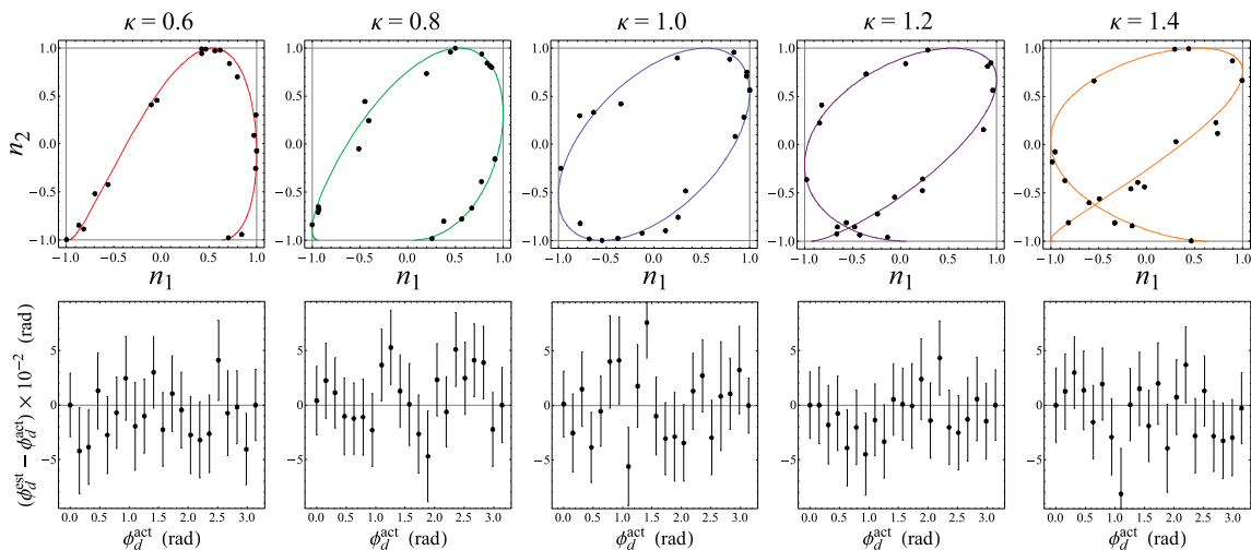
Figure B3. Simulated Bayesian phase estimates in the presence of differential phase noise. Top row: simulated data for \kappa = \{0.6, 0.8, 1.0, 1.2, 1.4\} . Similar to figure B2, common phases are randomly chosen over the range \phi_c \in [-\pi, \pi] , and the differential phase is set to \phi_d^{\text{act}} = 1 rad. Differential phase noise is applied to each point with a standard deviation of \sigma_{\phi_d} = 0.1 rad (SNR \sim 10 ). Bottom row: the systematic error in the Bayesian phase estimate, \phi_d^{\text{est}} - \phi_d^{\text{act}} , as a function of \phi_d^{\text{act}} for each value of \kappa . Only 10 points were required to bring the statistical uncertainty to \lesssim 50 mrad.
