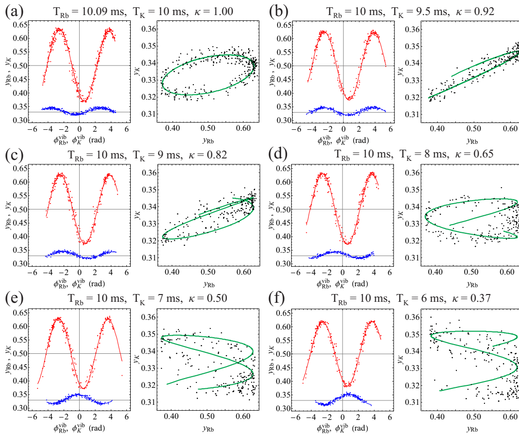
Figure 7. Correlation studies for different levels of temporal overlap. The symmetric, quasi-simultaneous K-Rb interferometer was operated with T_{\text{Rb}} = 10 ms and the interrogation time for potassium was varied between T_{\text{K}} = 6 - 10 ms. The interferometer phase was scanned by externally applied vibrations and individual fringes were restored using the FRAC method. Parametric plots of the atomic populations are shown to the right, along with the expected Lissajous curve (solid green line). These curves result from plotting the fit functions to each reconstructed fringe parametrically. There is a clear disagreement between the predicted Lissajous curves and the data for T_{\text{Rb}} - T_{\text{K}} \gtrsim 2 ms. Other interferometer parameters: \tau_{\text{Rb}} = \tau_{\text{K}} = 3 \mu\text{s} ; \Delta_{\text{Rb}} = \Delta_{\text{K}} \simeq -1.2 GHz.
