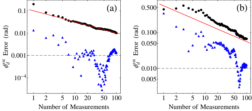
Figure B4. The statistical and systematic error in the Bayesian phase estimator as a function of the number of measurements, N , used in the Bayesian analysis for (a) differential phase noise and (b) offset noise. In both plots, \kappa = 0.8 , \phi_d^{\text{act}} = 1 rad, and M = 50 samples were used. Black points represent the statistical uncertainty \epsilon_{\phi_d}^{\text{stat}} , and blue triangles indicate the systematic error \epsilon_{\phi_d}^{\text{sys}} . The solid red lines indicate the minimum convergence rates based on \sigma_{\phi_d}/\sqrt{N} for differential phase noise and on 1/\sqrt{NI(\phi_d)} for offset noise, where I(\phi_d) is the Fisher information given by eq. (B.14). The dashed horizontal lines represent the nominal phase resolution used in the simulations. Values of \sigma_{\phi_d} = 0.1 rad (SNR \sim 10 ) and \sigma_{B_1} = \sigma_{B_2} = 0.2 (SNR \sim 5 ) were used as the noise parameters in (a) and (b), respectively.
