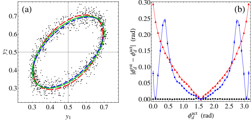
Figure A1. (a) Synthetic data following an ellipse with added offset noise. The solid green curve represents the actual ellipse, and fits to the data using the DEF method (red curve with big dashes) and FGEF method (blue curve with small dashes). The simulated ellipse contains 500 points with Gaussian-distributed noise on the offset parameters B_j with standard deviations \{\sigma_{B_1}, \sigma_{B_2}\} = \{0.01, 0.03\} (corresponding to \text{SNR} \sim \{20, 6\} ). Ellipse parameters: A_1 = A_2 = 0.2 , B_1 = B_2 = 0.5 , \kappa = 1 , \phi_d = 1 rad. (b) Measured bias in differential phase estimates, \phi_d^{\text{est}} , from the DEF (red triangles) and FGEF (blue points) methods relative to the actual value, \phi_d^{\text{act}} . The black squares show the estimates from the differential FRAC method for comparison. On all plots, the error bars correspond to the statistical distribution of fits to 100 synthetic data sets.
