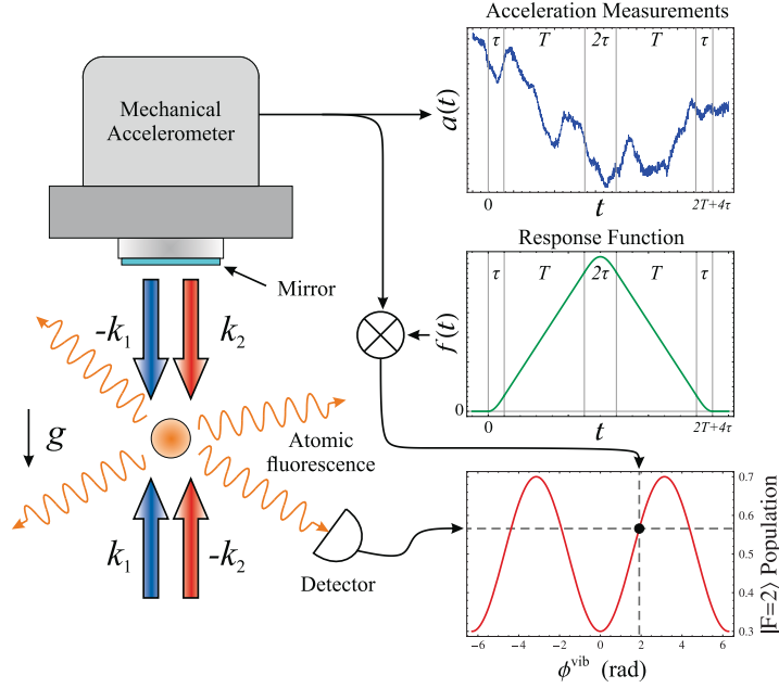
Figure 2. Schematic of the FRAC method for a single interferometer. A mechanical accelerometer is mounted to the back of the retro-reflection mirror for the Raman beam (with wave vectors k_1 and k_2 ). Acceleration measurements during the interferometer sequence are weighted by the response function f(t) [see eq. (C.5)] and integrated to obtain the phase estimate \phi^{\text{vib}} . Correlating this phase with the interferometer signal during the same time interval reproduces the interference fringe.
