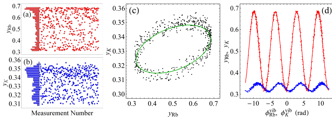
Figure 6. Measurements of normalized |F = 2\rangle state populations from simultaneous K-Rb interferometers operating at T \simeq 3 ms. Fringes are scanned randomly by applying vibrational noise to the retro-reflection mirror. Graphs (a) and (b) show a time series of 500 measurements from the ^{87}\text{Rb} and ^{39}\text{K} interferometers, respectively, along with histograms of the populations. (c) Atomic populations from (a) and (b) plotted parametrically—indicating strong correlation between the two species. The solid green line is an ellipse fit to the data using the FGEF method, which yields a differential phase \phi_d^{\text{ellipse}} = 1.13(2) rad. A separate estimate from a Bayesian analysis gives \phi_d^{\text{Bayes}} = 1.18(2) rad. (d) Interferometer fringes reconstructed from measurements of mirror motion using the FRAC method. The red and blue curves correspond to least-squares fits to Rb and K data, respectively. The differential phase estimated from the fits is \phi_d^{\text{FRAC}} = 1.17(1) rad. Other interferometer parameters: pulse separations: T_{\text{Rb}} = 3.018 ms, T_{\text{K}} = 3 ms; \pi/2 -pulse durations: \tau_{\text{Rb}} = 4 \mu\text{s} , \tau_{\text{K}} = 6 \mu\text{s} ; delay between interferometers: \Delta T_{\text{K,Rb}} = 10 \mu\text{s} ; one-photon Raman detunings: \Delta_{\text{Rb}} = \Delta_{\text{K}} \simeq -1.2 GHz.
