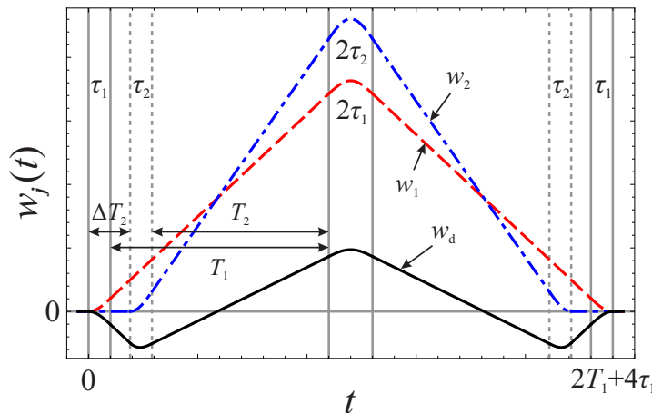
Figure C1. Weight functions, w_j(t) , described by the response function (C.5). These weights determine the phase shift associated with mirror vibrations in eq. (C.4). The pulse durations, \tau_j , satisfy \Omega_j^{\text{eff}}\tau_j = \pi/2 . The differential weight function, i.e. the difference between the red and blue curves, is shown in black.
