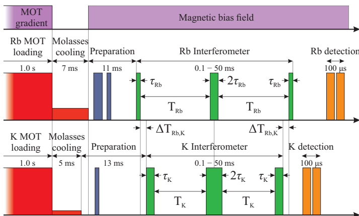
Figure 4. Symmetric timing sequence for the K-Rb interferometer. The first Raman pulse of the ^{39}\text{K} interferometer is delayed by \tau_{\text{Rb}} + \Delta T_{\text{Rb,K}} relative to that of ^{87}\text{Rb} such that the central \pi -pulse of both interferometers occurs at the same time. The preparation stages (shown in blue) include both the internal state preparation pulses (microwave + push beam for ^{87}\text{Rb} , depump for ^{39}\text{K} ), and the external state preparation via time-of-flight. Raman pulses are shown in green, and detection pulses in orange.
