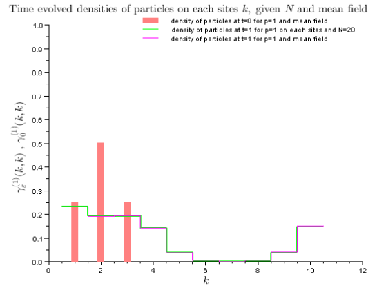
(f) Compared densities of particles at times t=0 and t=1
