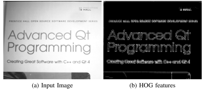
Fig. 8: HOG feature extraction
