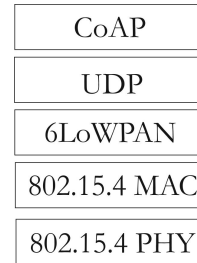
Fig. 4: Networking Stack
