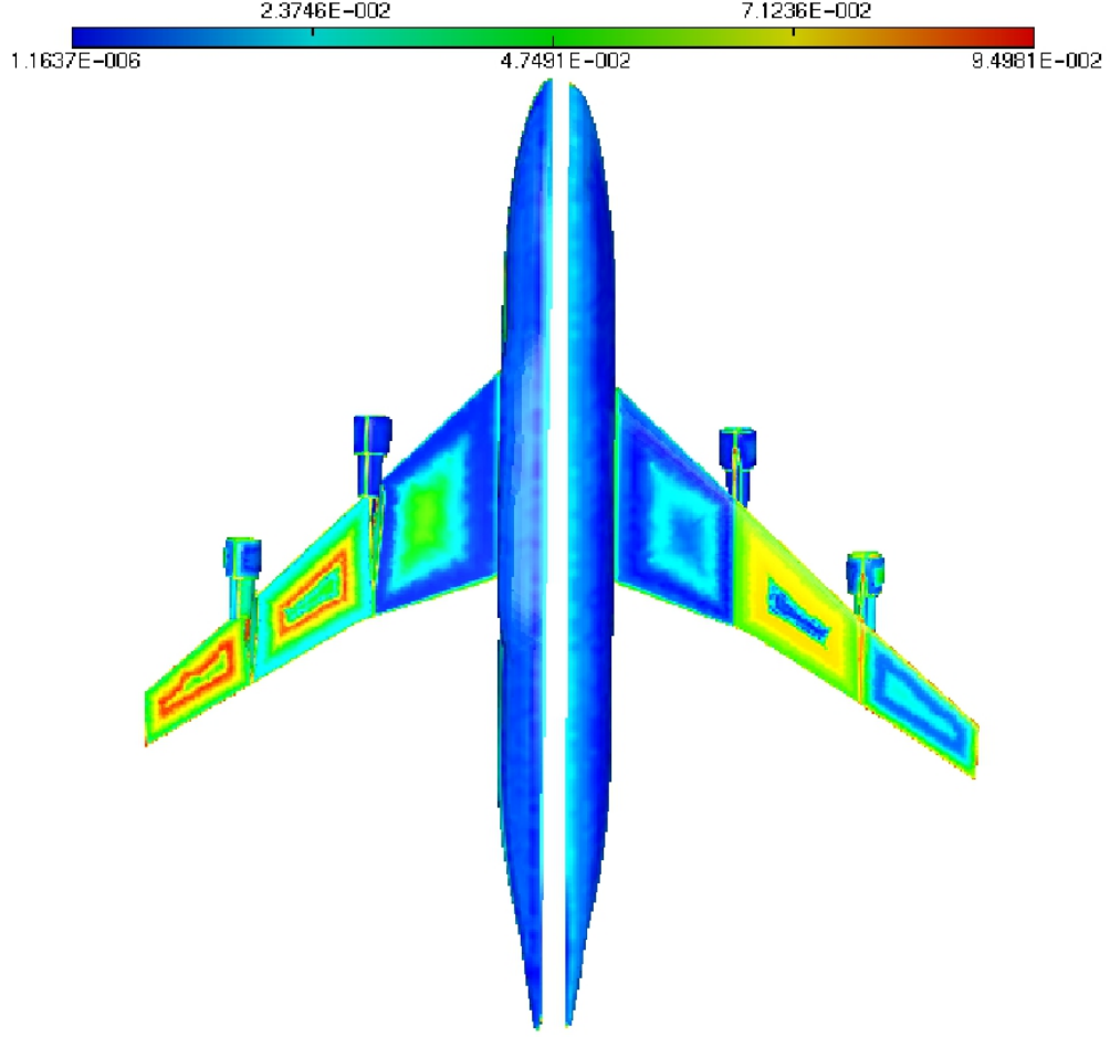
FIGURE 13. |diag(Cov_{\mathbf{x}})^{1/2} - diag(Cov_{\mathbf{x}^{\pm}})^{1/2}| (meter) on the lower (left) and upper (right) surfaces of the aircraft.
