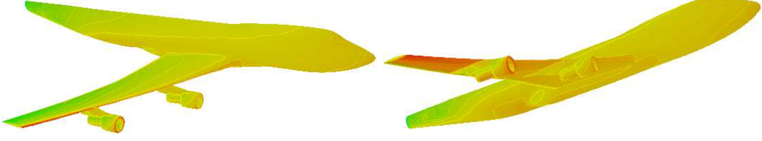
FIGURE 8. p^* \sigma^2 \frac{\partial j / \partial p^*}{\|\partial j / \partial p^*\|} to build directional extreme scenarios with (25).
