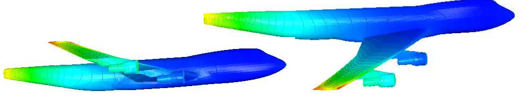
FIGURE 10. Assumption of Cov_{p^*}(= p^* \sigma^2 I) used in getting Cov_{\mathbf{x}} from (26).
