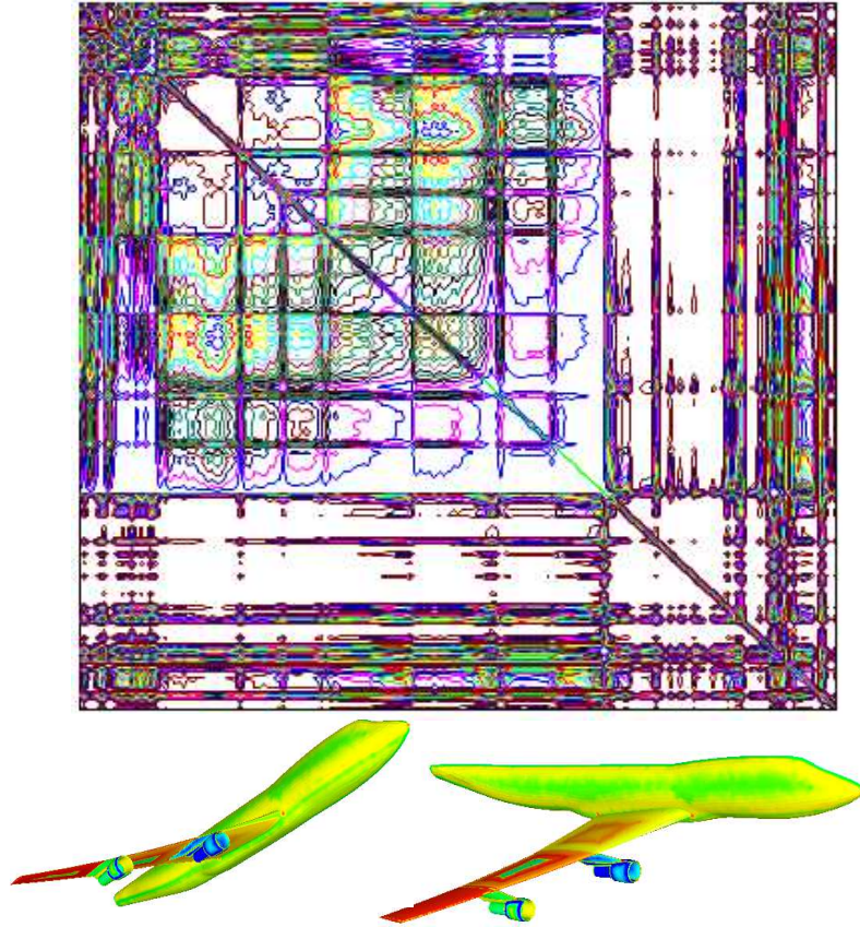
FIGURE 11. Graph of Cov_{\mathbf{x}} from (26). This is a n \times n = 16K \times 16K matrix. Three main regions of interaction (wing, wing-body, tail) can be identified. Iso-contours show an example of correlations in the design parameters between a point in the wing tip region and the rest of the aircraft (this is a line of Cov_{\mathbf{x}} ).
