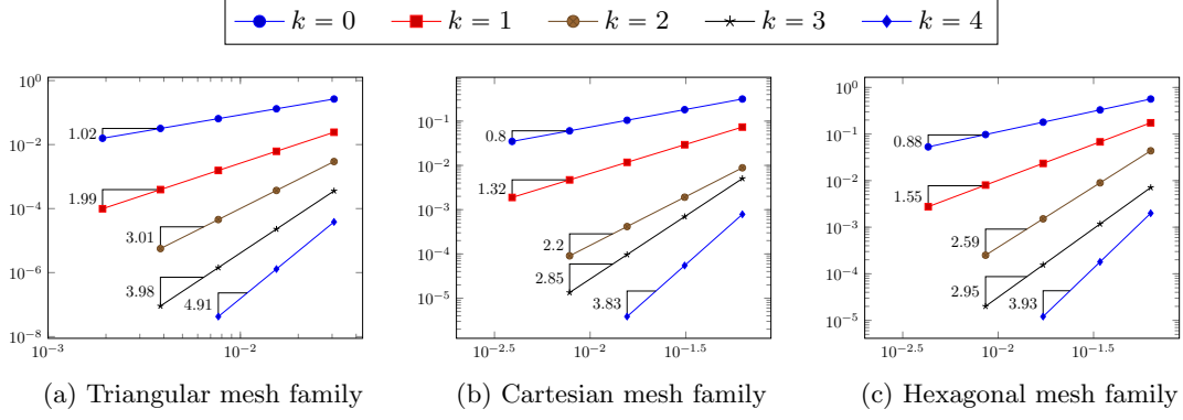
Figure 5: \|\mathbf{G}_h^k(\underline{\mathbf{u}}_h - I_h^k u)\|_{L^p(\Omega)^d} vs. h , p = 4 for the variant of the method discussed in Remark 4.4 and corresponding to l = k + 1 .
