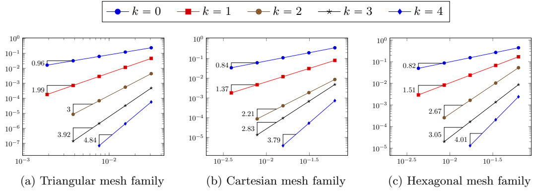
Figure 4: \|\mathbf{G}_h^k(\underline{u}_h - \mathbb{I}_h^k u)\|_{L^p(\Omega)^d} vs. h , p = 4 .
