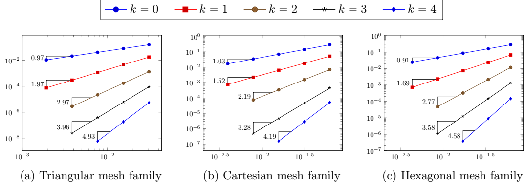
Figure 3: \|\mathbf{G}_h^k(\underline{u}_h - \mathbb{I}_h^k u)\|_{L^p(\Omega)^d} vs. h , p = 3 .
