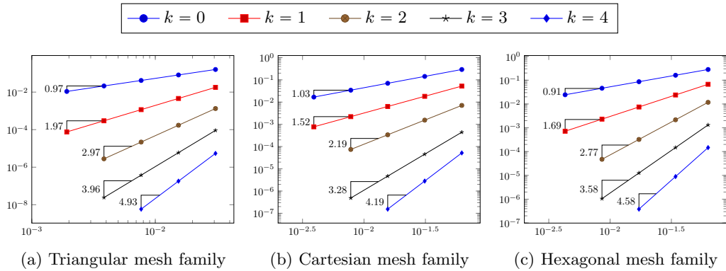
Figure 3: \|G_h^k(\underline{u}_h - \mathbb{1}_h^k u)\|_{L^p(\Omega)^d} vs. h , p = 3 .
