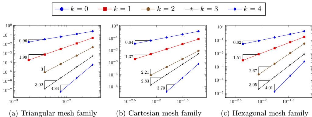
Figure 4: \|G_h^k(\underline{u}_h - \mathbb{1}_h^k u)\|_{L^p(\Omega)^d} vs. h , p = 4 .
