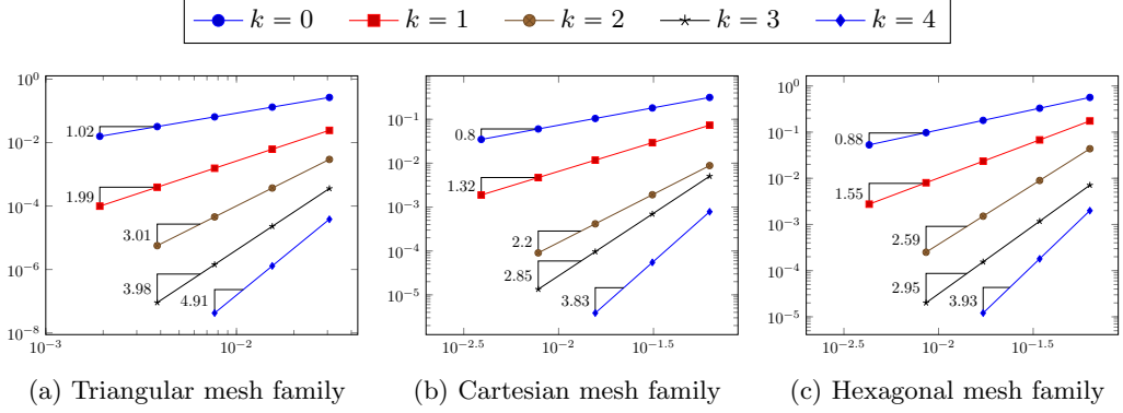
Figure 5: \|G_h^k(\underline{u}_h - \underline{I}_h^k u)\|_{L^p(\Omega)^d} vs. h , p = 4 for the variant of the method discussed in Remark 4.3 and corresponding to l = k + 1 .
