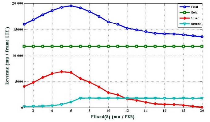
Fig. 3. Mean revenue versus P_{fixed}(S) when using R2P
