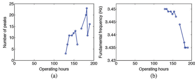
Figure 4. Evolution of (a) the number of peaks and (b) the fundamental frequency of the harmonic series representing the BPFI of the test-rig main bearing
