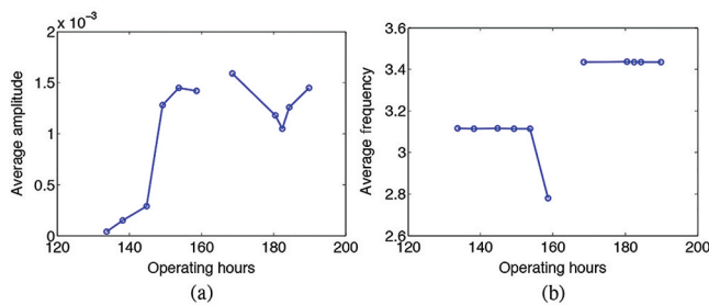
Figure 5. Evolution of the shaft speed (0.333 Hz) modulations around the BPFI (3.45 Hz) carrier frequency: (a) average of the amplitude modulation function; (b) average of the frequency modulation function
