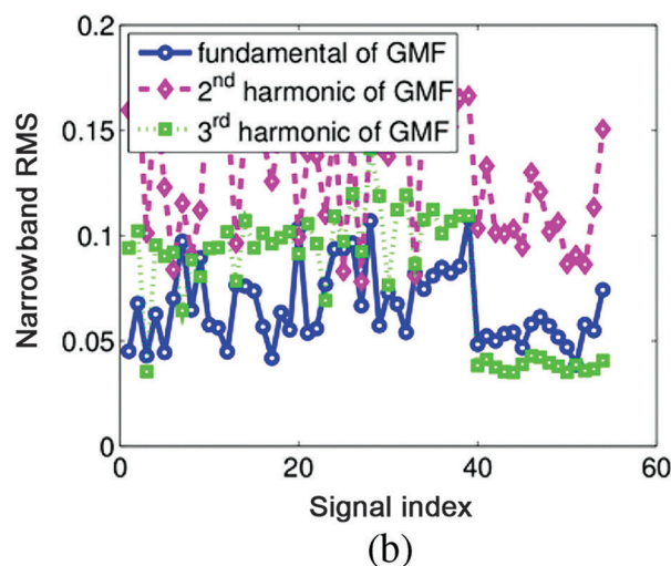
Figure 10. Diagnosis of the anonymous wind turbine gearbox: (a) frequency modulation index obtained in AStrion by demodulating the side-band series around the second harmonic of GMF modulated by shaft speed; and (b) narrowband RMS computed with a bandwidth of three side-bands on both sides of the carrier frequency
