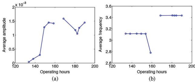
Figure 5. Evolution of the shaft speed (0.333 Hz) modulations around the BPF (3.45 Hz) carrier frequency: (a) average of the amplitude modulation function; (b) average of the frequency modulation function
