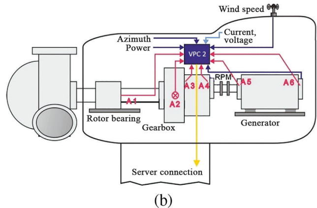
Figure 6. (a) The geographical location of the wind turbine WT6 and (b) the accelerometers A5 and A6 installed, respectively, at the front and the rear end of the generator
