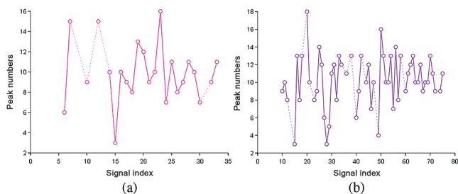
Figure 9. Evolution of the number of peaks in the harmonic series associated with the shaft speed: (a) accelerometer A5; (b) accelerometer A6
