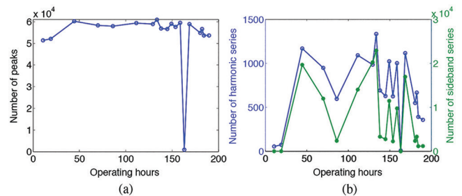
Figure 3. Results of the detection of peaks, harmonic series and side-band series on the 19 signals of accelerometer (+y), mounted on the main bearing of the test-rig from 10.62 to 189.85 operating hours: (a) number of peaks detected; and (b) number of harmonic and side-band series detected
