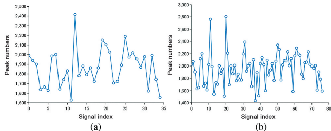
Figure 8. Evolution of the number of detected peaks for both accelerometers: (a) accelerometer A5; (b) accelerometer A6
