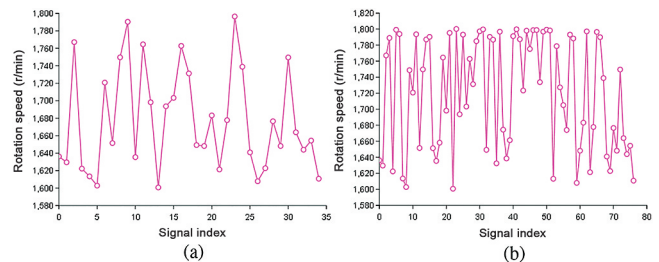
Figure 7. Evolution of the mean rotational speed: (a) accelerometer A5; (b) accelerometer A6
