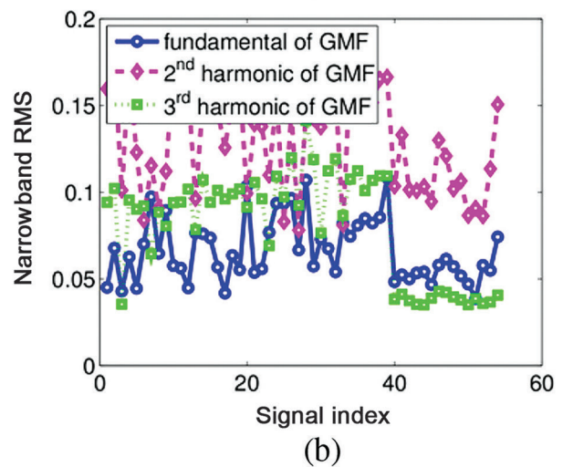
Figure 10. Diagnosis of the anonymous wind turbine gearbox: (a) frequency modulation index obtained in AStrion by demodulating the side-band series around the second harmonic of GMF modulated by shaft speed; and (b) narrowband RMS computed with a bandwidth of three side-bands on both sides of the carrier frequency
