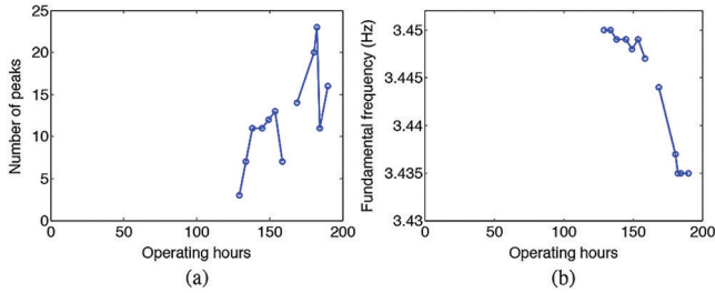
Figure 4. Evolution of (a) the number of peaks and (b) the fundamental frequency of the harmonic series representing the BPF of the test-rig main bearing
