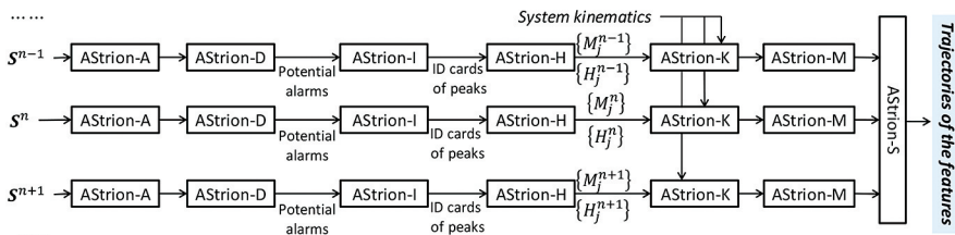
Figure 1. The modular architecture of AStrion
