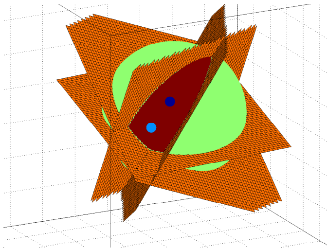
Fig. 1: An Example of version space where the Chebyshev Center (light blue) is a bad approximation of the gravity center (dark blue).
