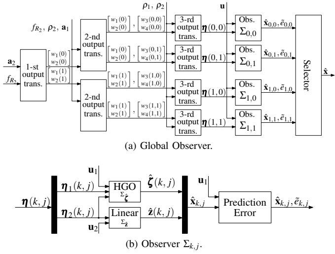
Fig. 2: Graphic representation of the observer.
