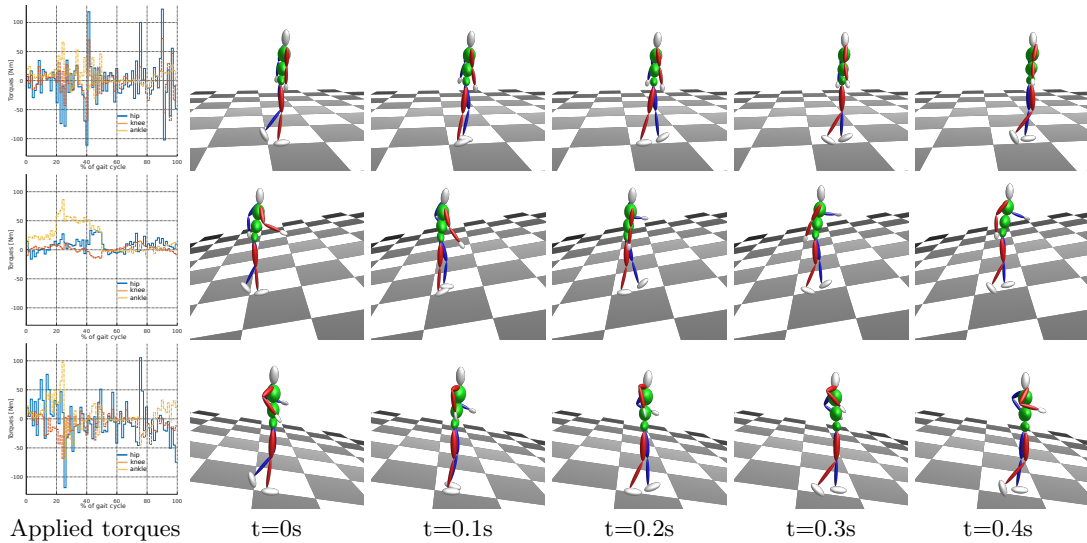
Figure 2: Curves showing the torques for the hip, knee and ankle joints of the right leg and snapshots of the three walking movements: flat ground, tilt of +10 deg and tilt of -10 deg.
