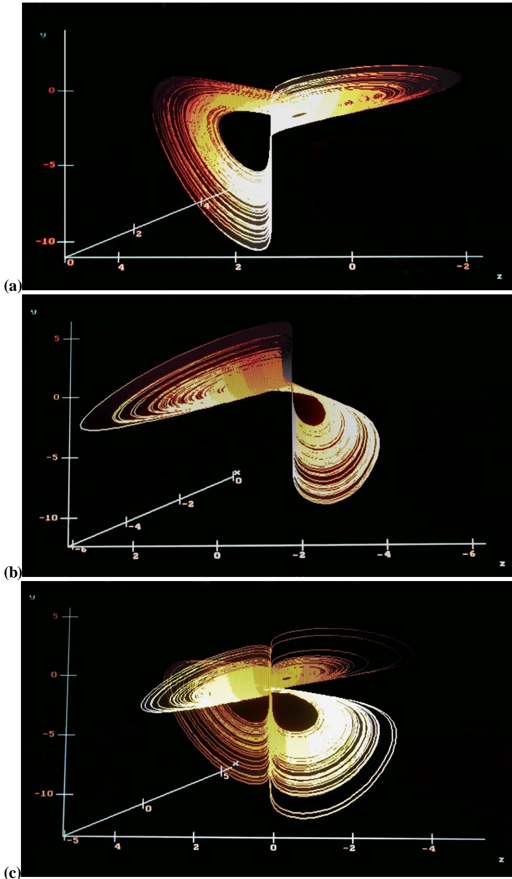
Fig.4. Portraits of the attractor for C_2(2, -3, 0.8, 1, -2, 3) in the phase space (z, y, x) . (a) The attractor appears in the positive domain of the x -axis, (b) the attractor located in the negative part of the x -axis, and (c) the disposition of the two chaotic trajectories gathered in the same representation.
