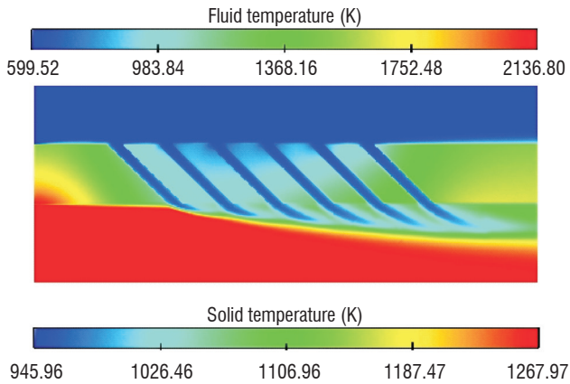
Figure 5 - Temperature field
