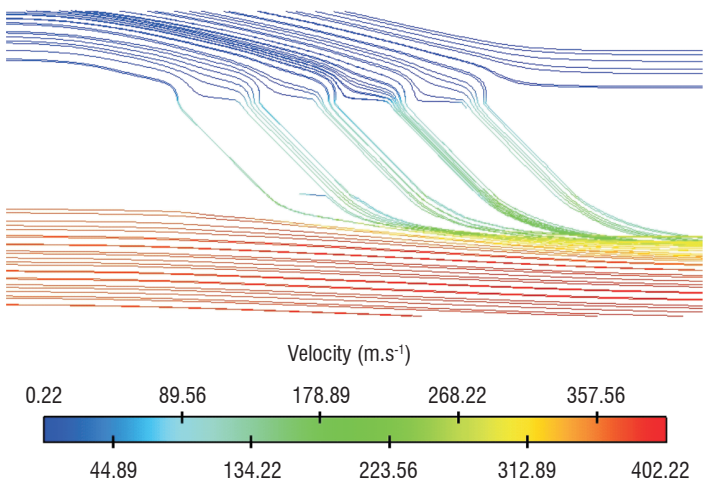
Figure 6 - Velocity streamlines
